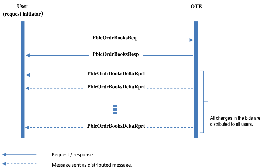
Picture 10 - Sequential scheme of bid request processing
