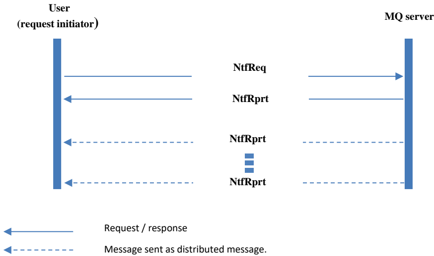
Picture 122 - Sequential scheme of notification messages request processing
