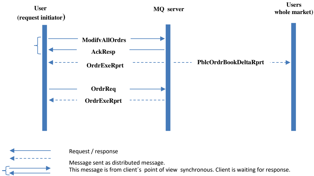
Picture 6 - Sequential scheme of mass bid modification (deactivation) and subsequent request for bids
