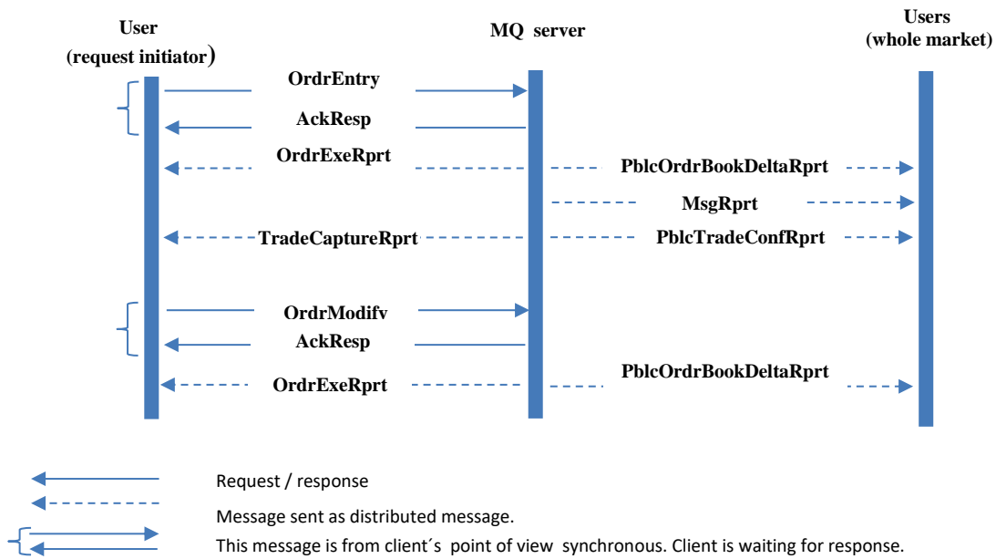
Picture 4 – Sequential scheme of bid entry with its trading and bid modification without trade creation
