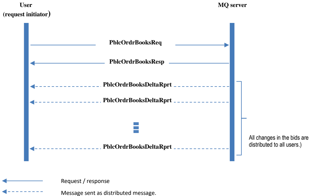
Picture 7 - Sequential scheme of bid request processing
