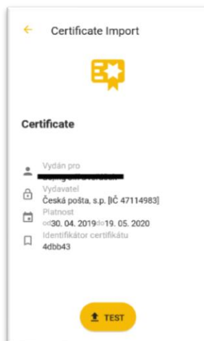
Obr. 15 –Certificate import
